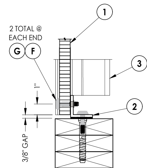
SECTION @ MULLION END
