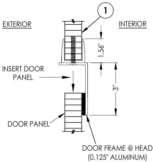
2 VERTICAL CROSS SECTION
