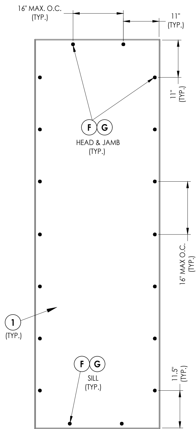
EXTERIOR VIEW SINGLE PANEL ANCHORING SHUTTER PANEL TO ALUMINUM BRACKET
