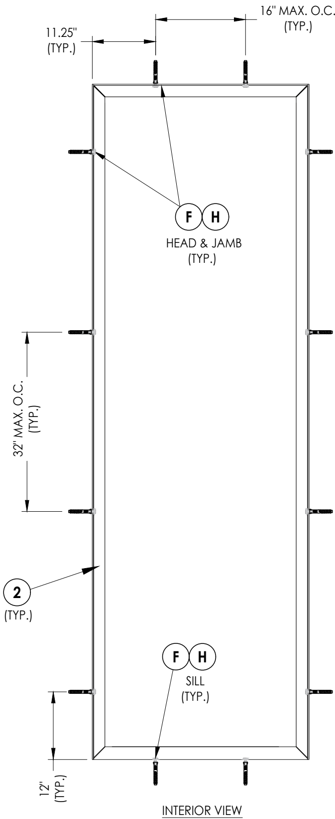
SINGLE PANEL FRAME ANCHORING ALUMINUM BRACKET TO MASONRY
