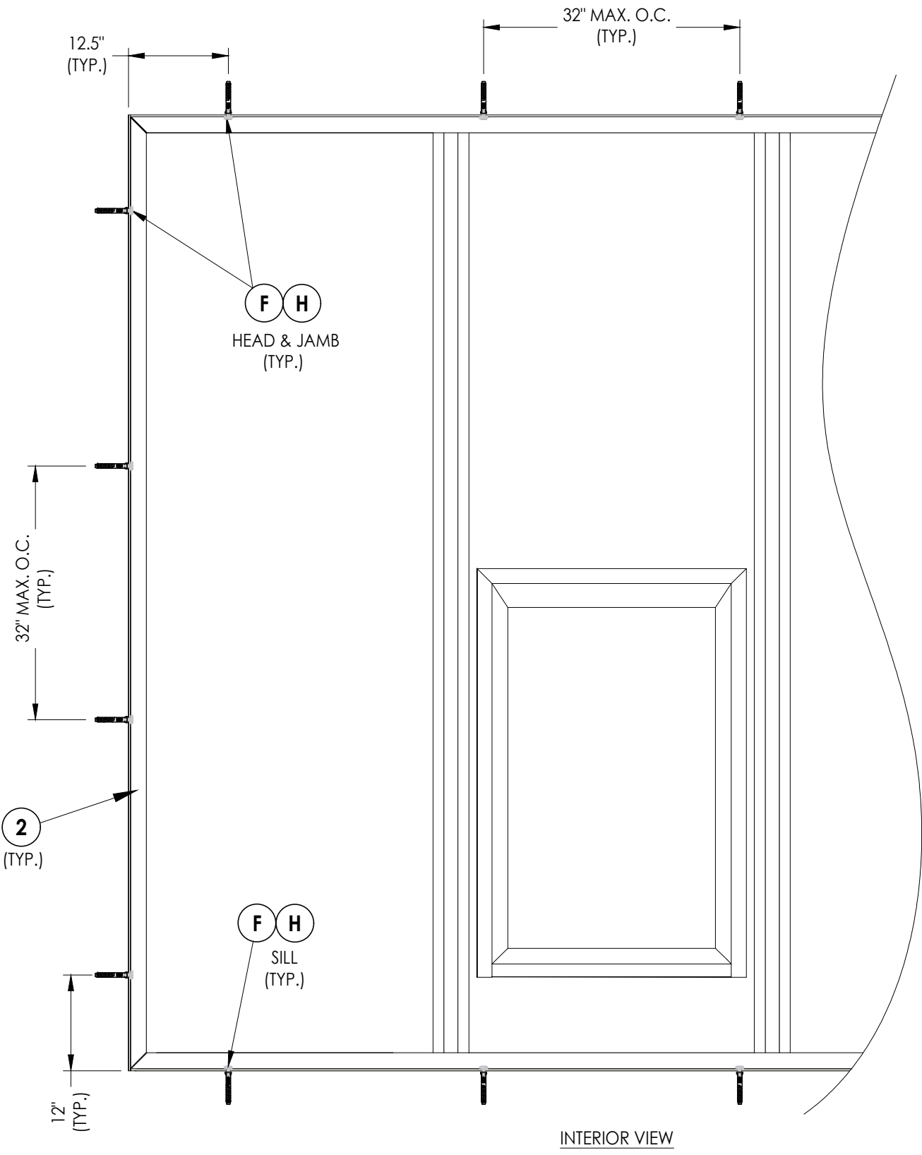
MULTIPLE PANEL FRAME ANCHORING ALUMINUM BRACKET TO MASONRY
