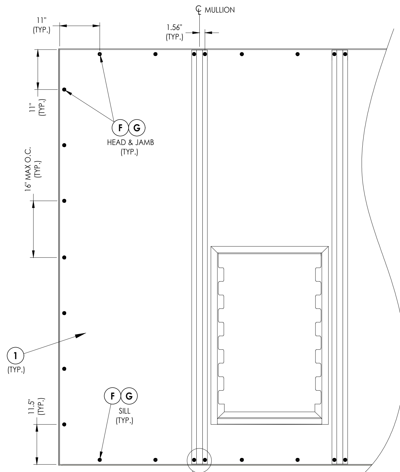
EXTERIOR VIEW MULTIPLE PANEL ANCHORING SHUTTER PANEL TO ALUMINUM BRACKET
